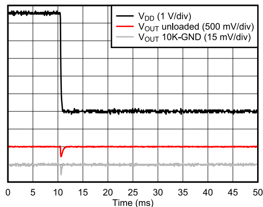
Figure 6-40. Power-off Glitch
