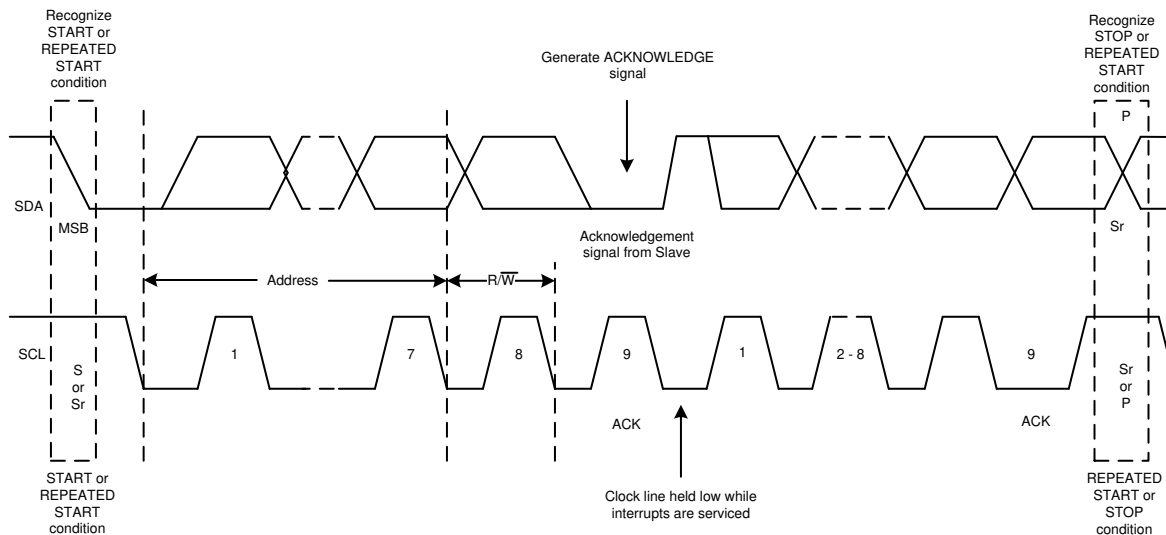
Figure 7-5. I²C Bus Protocol
