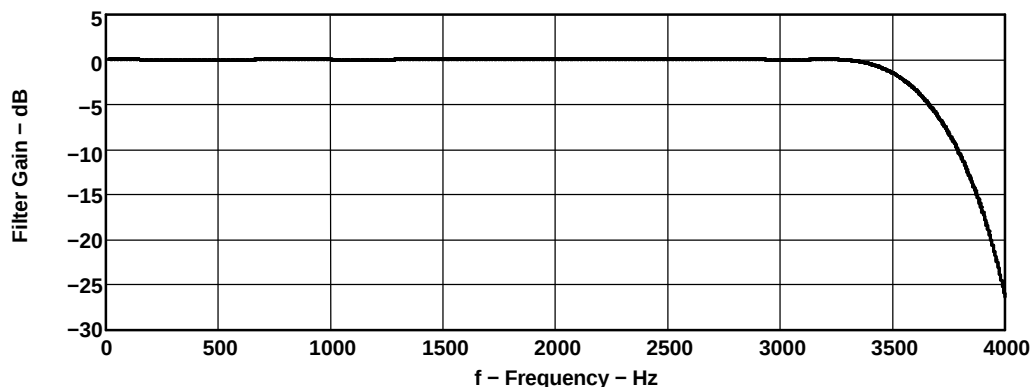
Figure 10. ADC FIR Frequency Response - HPF Off
