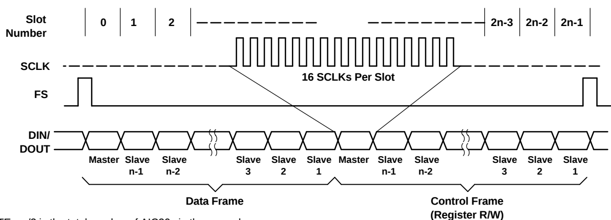
Figure 24. Standard Operation/Programming Mode: Master-Slave Cascade Timing
