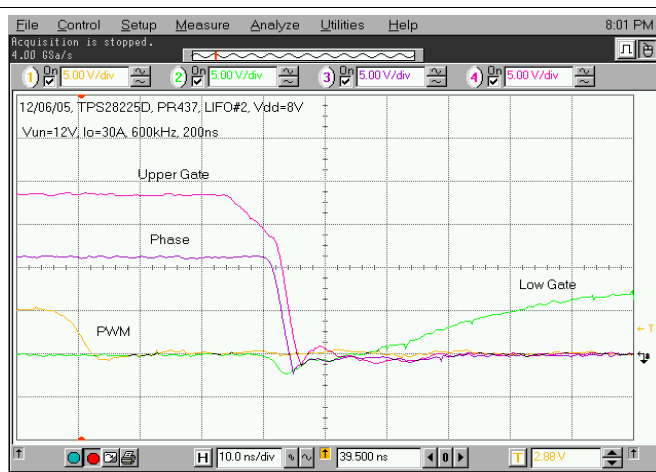
Figure 40. Phase Falling-Edge Switching Waveforms (10 ns/div) of the Power Stage in Figure 25
