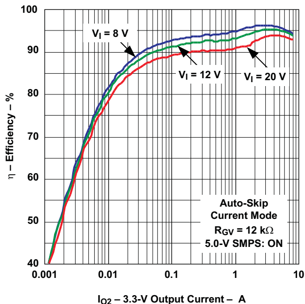
3.3-V EFFICIENCY vs OUTPUT CURRENT
