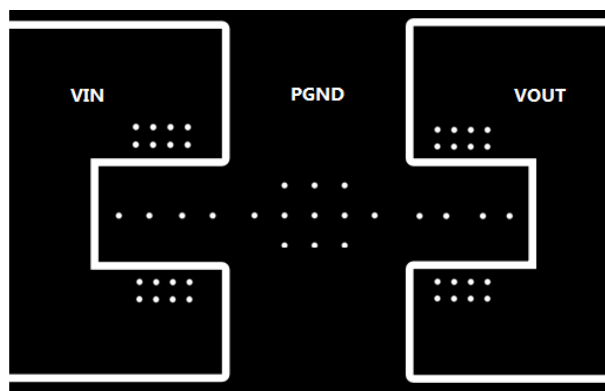
Figure 11-3. Typical Mid-Layer
