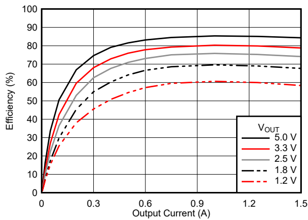
Figure 7-12. Efficiency
