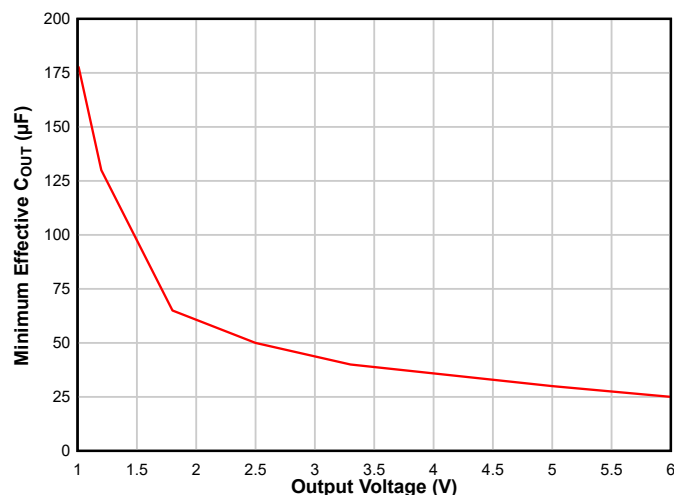
Figure 8-2. Minimum Required Output Capacitance
