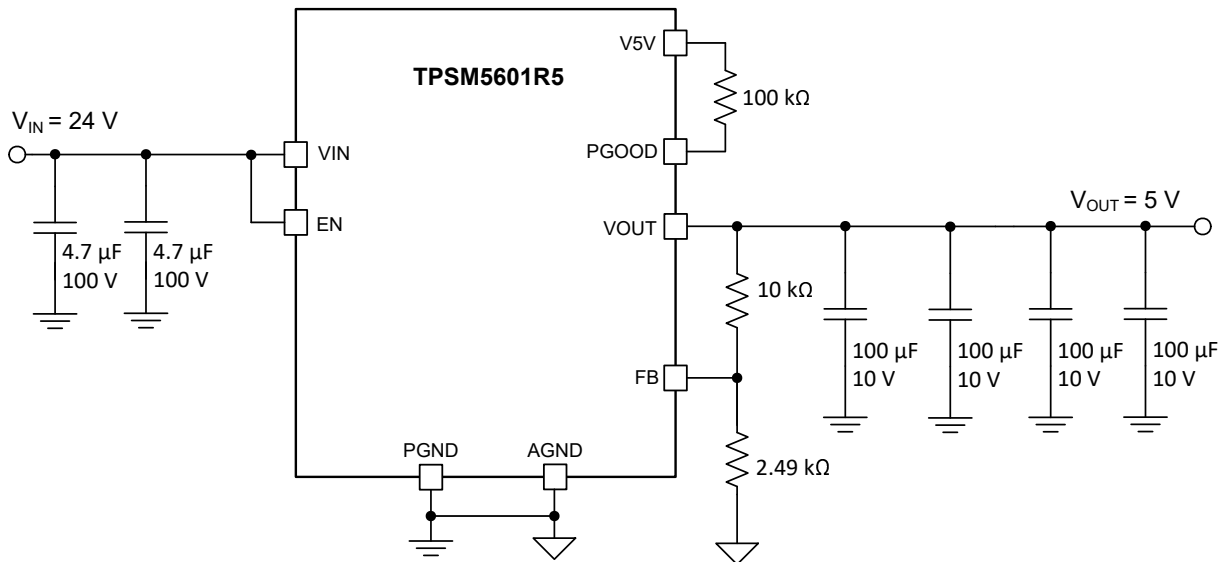
Figure 9-1. TPSM5601R5 Typical Schematic
