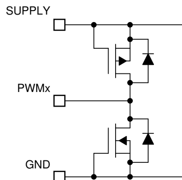
Figure 6-9. PWMx Pins
