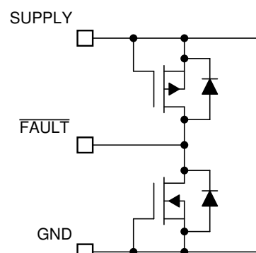
Figure 6-11. FAULT Pin
