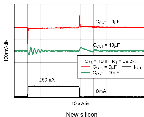
Figure 5-52. TPS73201-Q1 Load Transient, Adjustable Version
