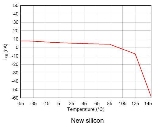
Figure 5-50. TPS73201-Q1 I_{FB} vs Temperature
