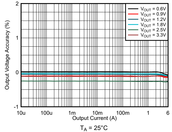
Figure 8-21. Load Regulation V_{IN} = 5.0\text{ V} and FPWM
