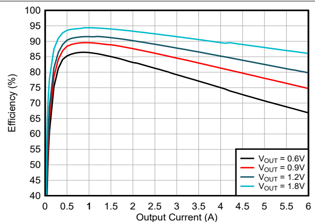
Figure 8-5. Efficiency V_{IN} = 3.3\text{ V} and T_A = 85^\circ\text{C}
