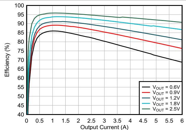
Figure 8-3. Efficiency V_{IN} = 5.0\text{ V} and T_A = 85^\circ\text{C}
