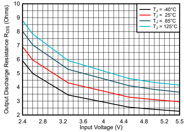
Figure 6-3. Output Discharge Resistance R_{DS}
