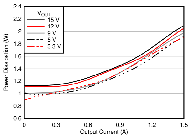
Figure 7-14. Power Dissipation
