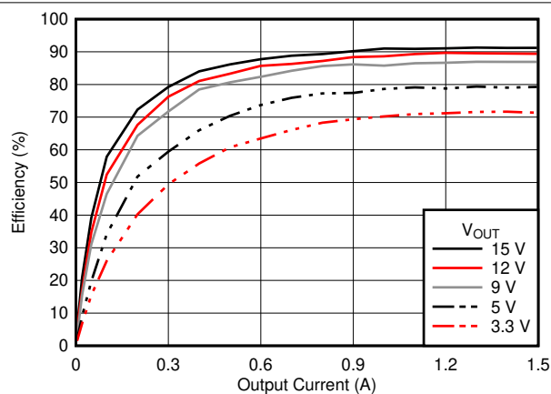
Figure 7-13. Efficiency
