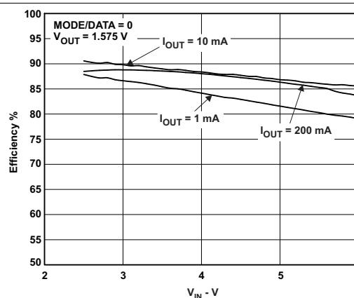
Figure 21. Efficiency TPS62403 VOUT1/VOUT2
