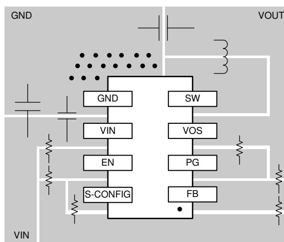
Figure 11-1. TPS629210E Layout
