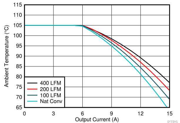
Figure 6-6. SOA, 5V IN 1.0V OUT , 600 KHz, FCCM, Internal VCC LDO
