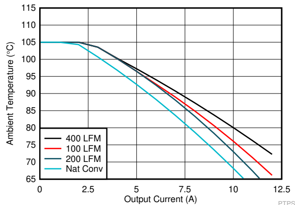
Figure 6-5. SOA, 12 V 5.0V OUT , 600 KHz, FCCM, Internal VCC LDO
