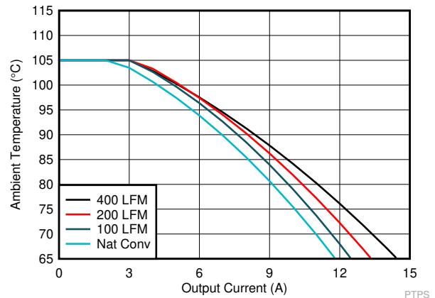
Figure 6-4. SOA, 12 V 3.3V OUT , 600 KHz, FCCM, Internal VCC LDO
