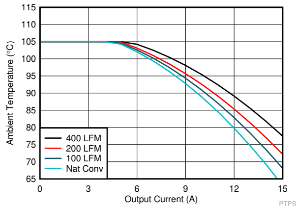
Figure 6-3. SOA, 12 V 1V OUT , 600 KHz, FCCM, Internal VCC LDO
