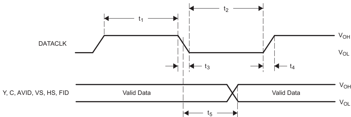
Figure 3-1. Clocks, Video Data, and Sync Timing
