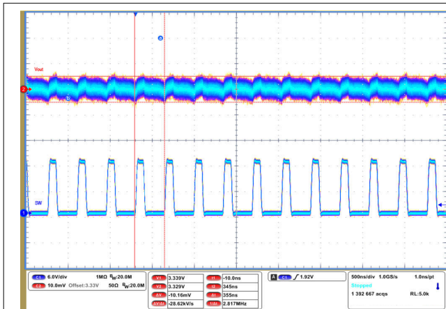
Figure 9-74. Output Voltage Ripple
