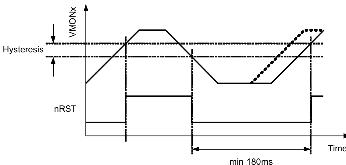
Figure 1. Supply Voltage Supervisor Reset Generation
