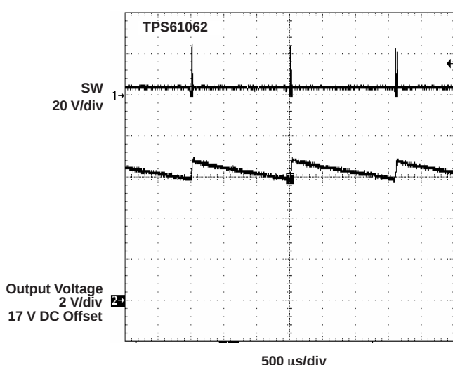
Figure 15. Overvoltage Protection
