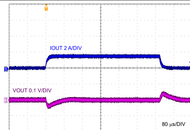
Figure 9-14. Load Transient, 0 A to 1.5 A
