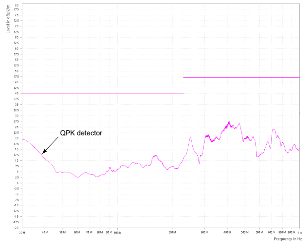
Figure 9-9. CISPR 32 Class B Radiated Emissions: Vertical Polarization
