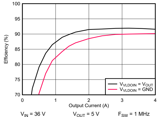
Figure 8-6. Efficiency Increase With External Bias
