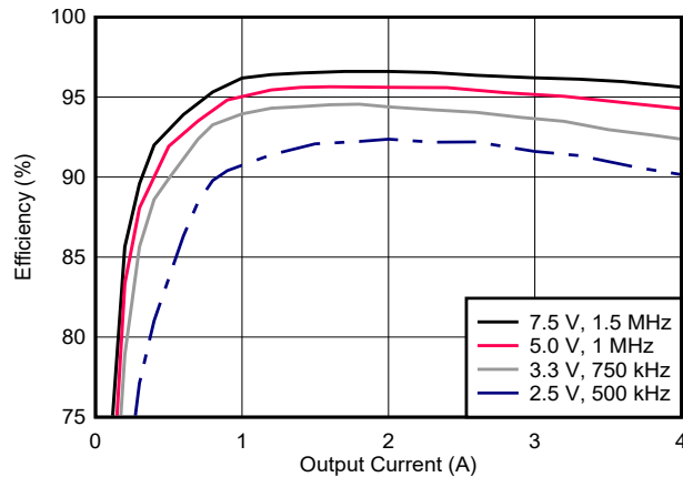
Figure 7-9. Efficiency
