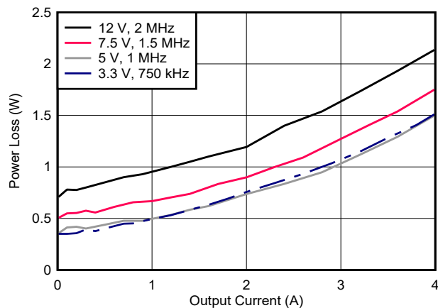
Figure 7-15. Power Dissipation
