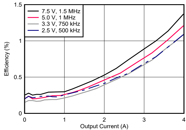
Figure 7-10. Power Dissipation
