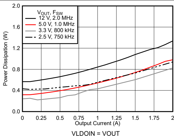
Figure 7-12. Power Dissipation
