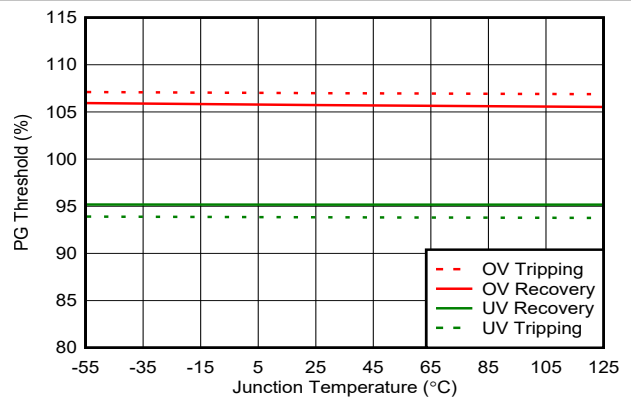
Figure 7-6. Power-Good (PG) Thresholds
