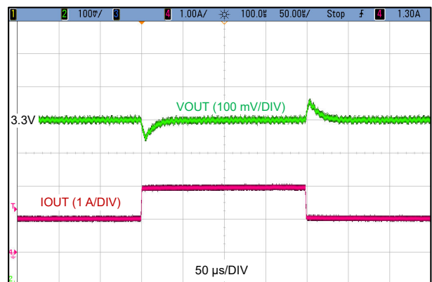
Figure 9-5. Load Transient, 1 A to 2 A, 1 A/μs
