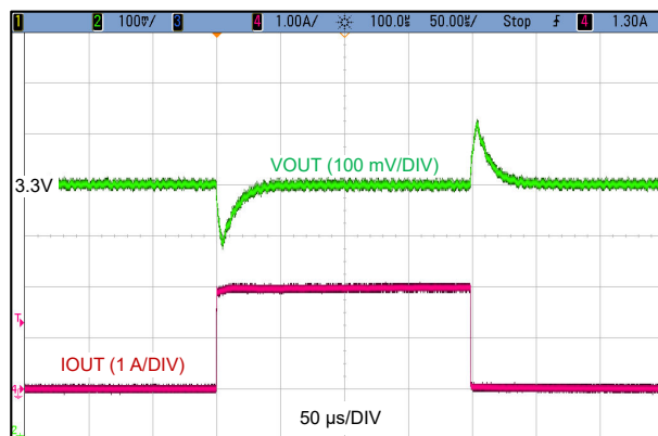
Figure 9-4. Load Transient, 0 A to 2 A, 1 A/μs
