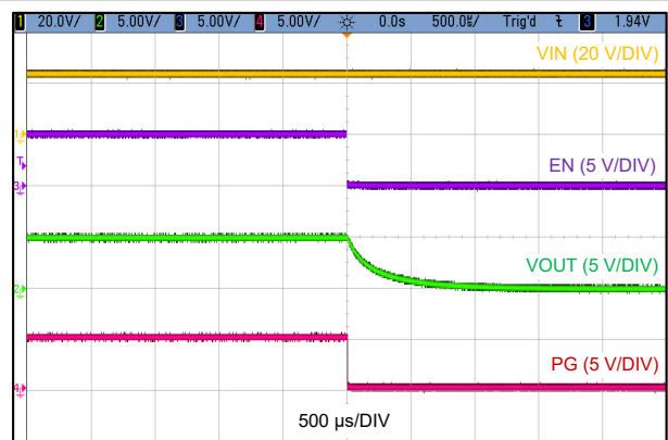
Figure 9-3. Shutdown Waveforms
