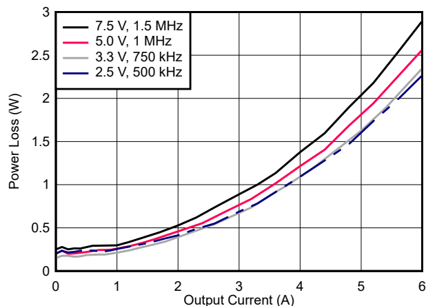
Figure 7-10. Power Dissipation
