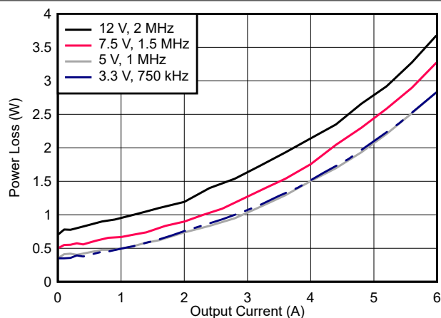
Figure 7-15. Power Dissipation
