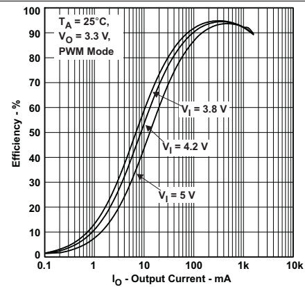
Figure 2. DCDC1: Efficiency vs Output Current
