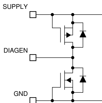
Figure 7-9. DIAGEN Pin
