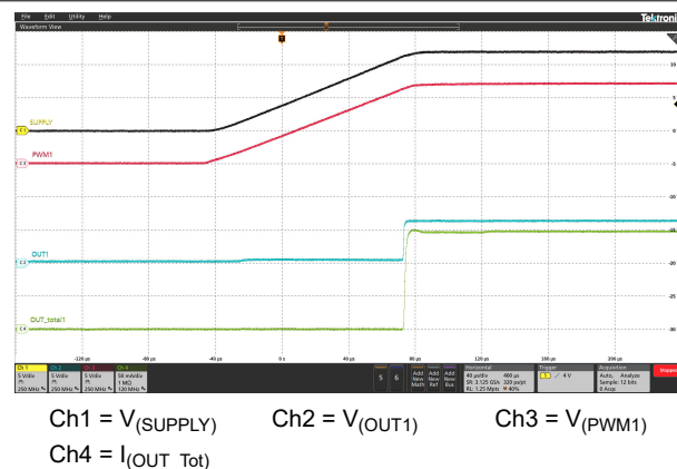
Figure 6-10. Power Up Sequence
