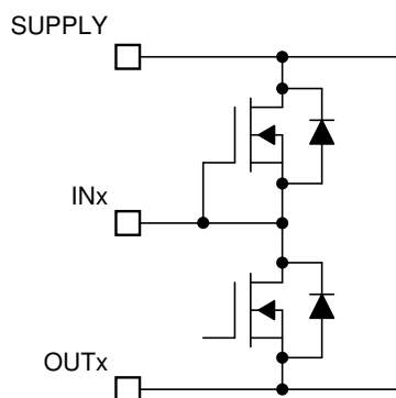
Figure 7-13. INx Pins
