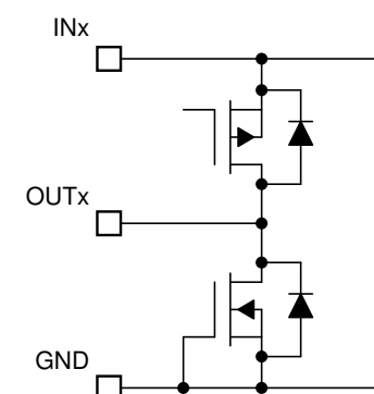
Figure 7-11. OUTx Pins
