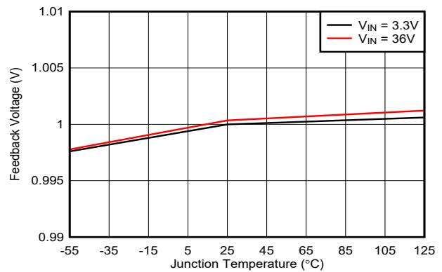
Figure 7-2. Feedback Voltage
