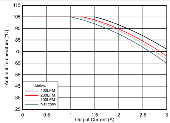
Figure 6-18. Safe Operating Area
