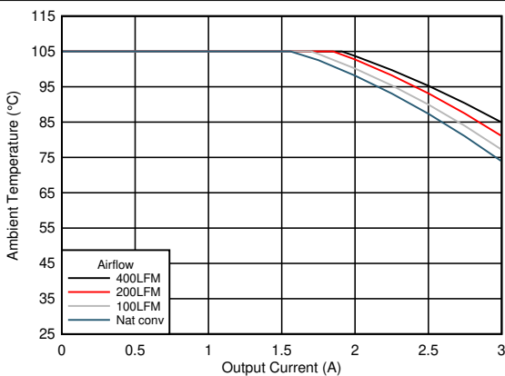
Figure 6-17. Safe Operating Area
