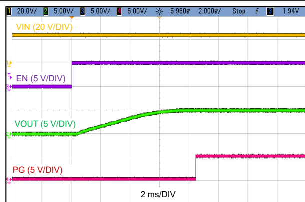
Figure 8-2. Start-Up Waveforms
