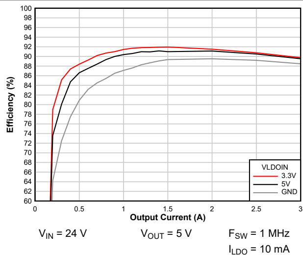
Figure 7-8. Efficiency improvements with VLDOIN ( V_{OUT} = 5\text{ V} )
