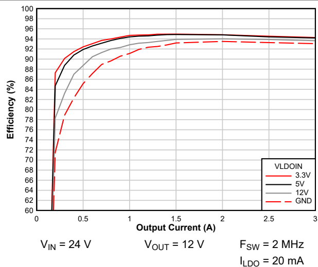
Figure 7-9. Efficiency improvements with VLDOIN ( V_{OUT} = 12\text{ V} )
