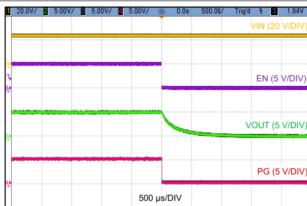
Figure 8-3. Shutdown Waveforms
