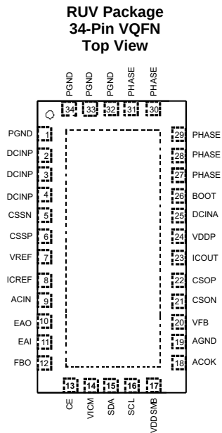
Pin Functions
