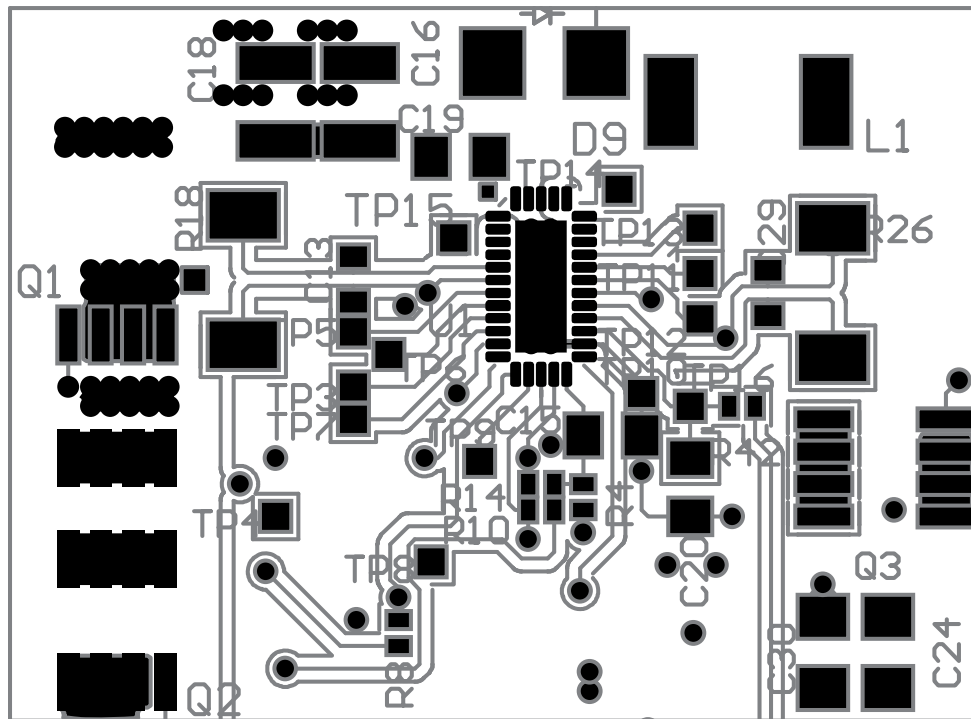
Figure 32. bq24765 Board Layout
