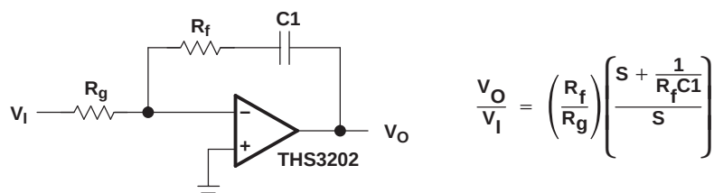
Figure 85. Inverting CFB Integrator
