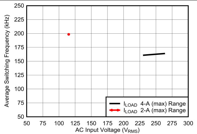
Figure 8-7. Average Switching Frequency at Full-Load vs. AC Input Voltage
