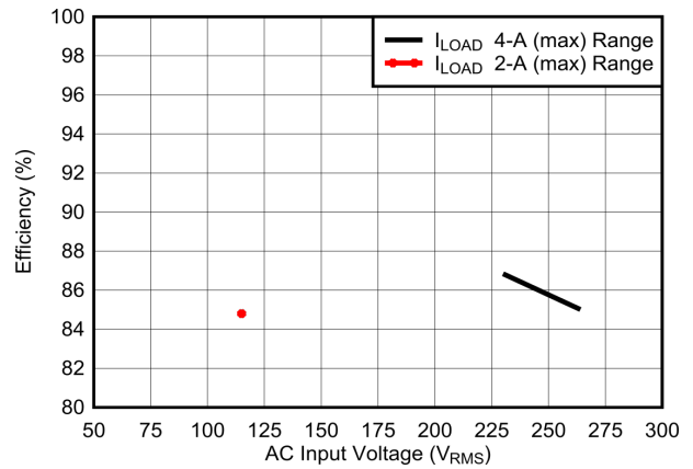
Figure 8-5. 10%-Load Efficiency vs. AC Input Voltage
