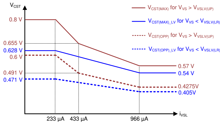
Figure 7-43. V_{CST} OPP curve across I_{VSL}
