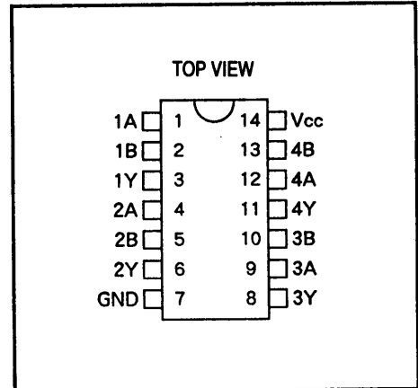
PIN ASSIGNMENT
