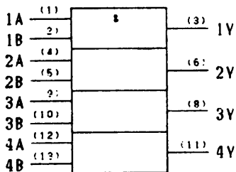
LOGIC SYMBOL
