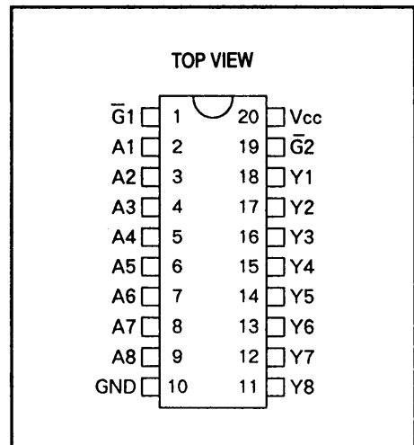
PIN ASSIGNMENT
