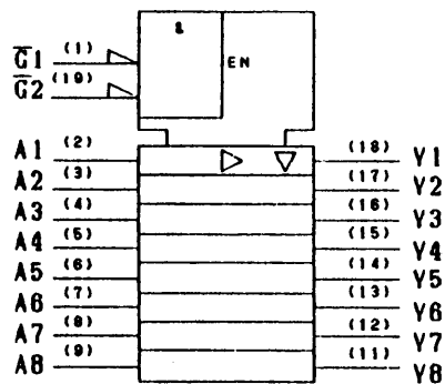
LOGIC SYMBOL
