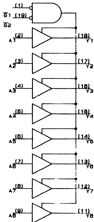
LOGIC DIAGRAM
