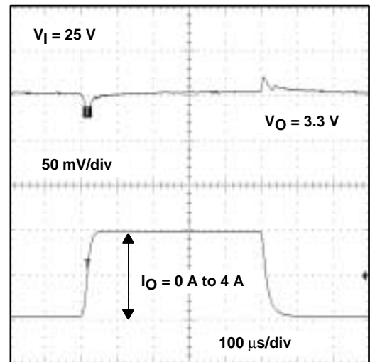
3.3 V OUTPUT VOLTAGE LOAD TRANSIENT RESPONSE
