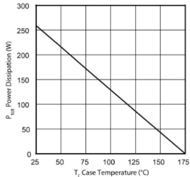
Figure 4 • Max Power Dissipation vs. Case Temp
