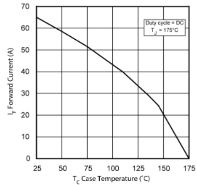
Figure 3 • Max Forward Current vs. Case Temp
