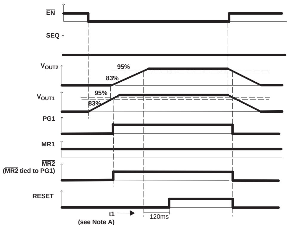
Figure 40. Timing when \text{SEQ} = \text{Low}
