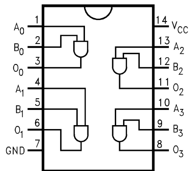
Figure 1. Pin Assignments for SOIC, SOP and TSSOP
