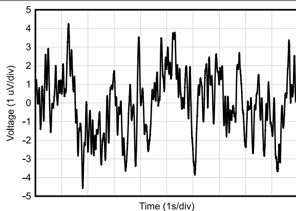
Figure 5-17. 0.1-Hz to 10-Hz Noise
