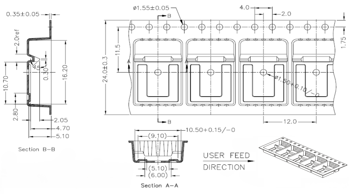
Figure 20. D 2 PAK tape drawing
