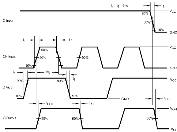
Figure 7. AC Waveforms
