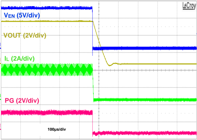
Figure 30. Shutdown Using EN with PG, IOOUT = 3.5A
