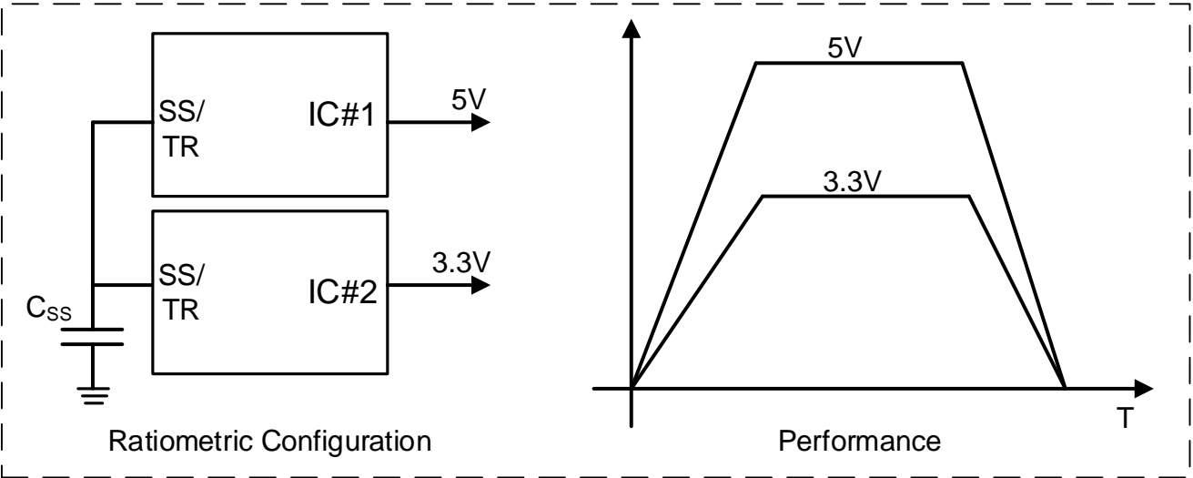
Figure 50. Ratiometric Configuration
