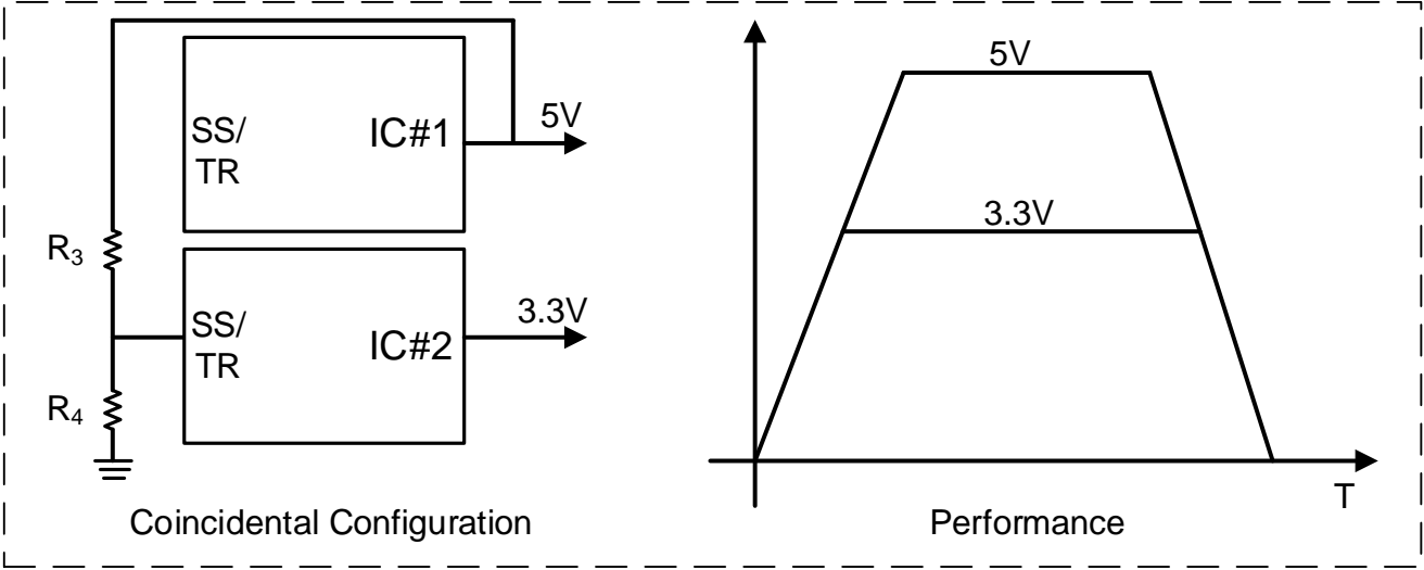
Figure 51. Coincidental Configuration
