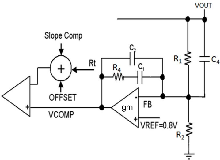
Figure 60. Type 2 Compensator
