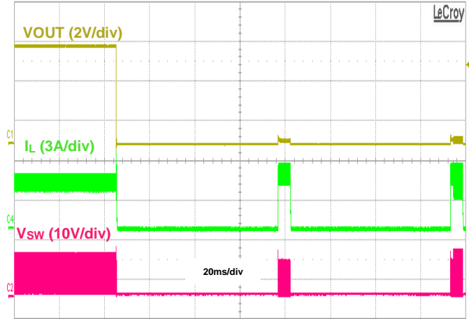
Figure 31. Output Short Protection, IOOUT = 3.5A
