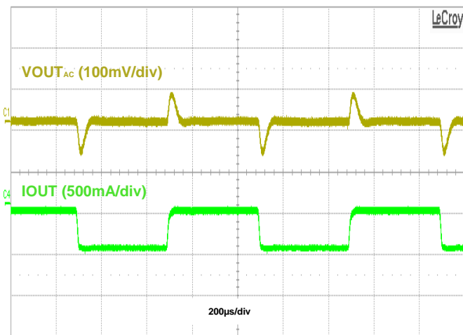
Figure 37. Load Transient, I_{OUT} = 50\text{mA} to 500\text{mA} to 50\text{mA} , PWM
