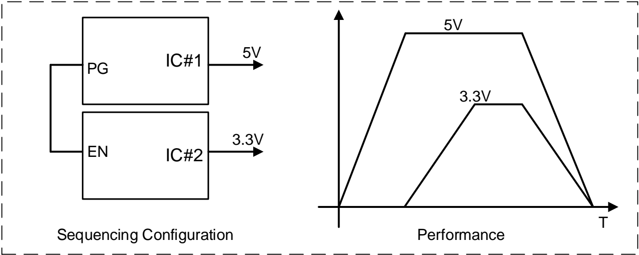
Figure 52. Sequencing Configuration
