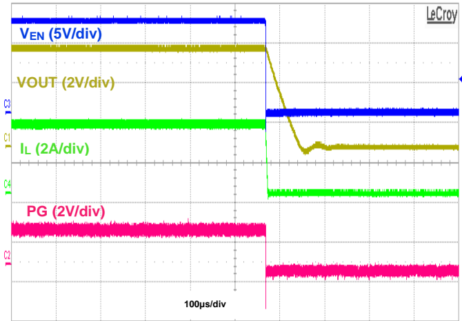
Figure 46. Shutdown Using EN with PG, I_{OUT} = 3.5\text{A}
