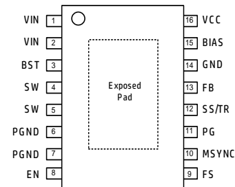
TSSOP-16EP (Top View)
