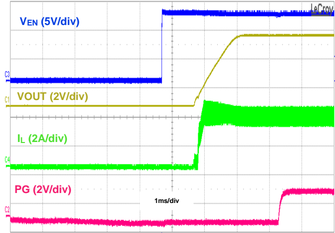
Figure 29. Startup Using EN with PG, IOOUT = 3.5A
