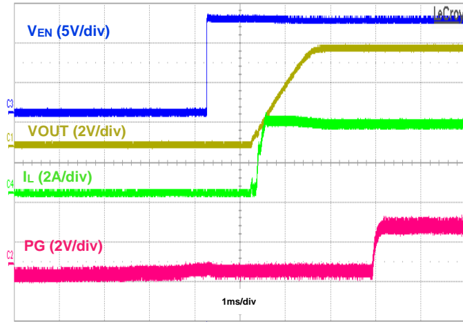
Figure 45. Startup Using EN with PG, I_{OUT} = 3.5\text{A}
