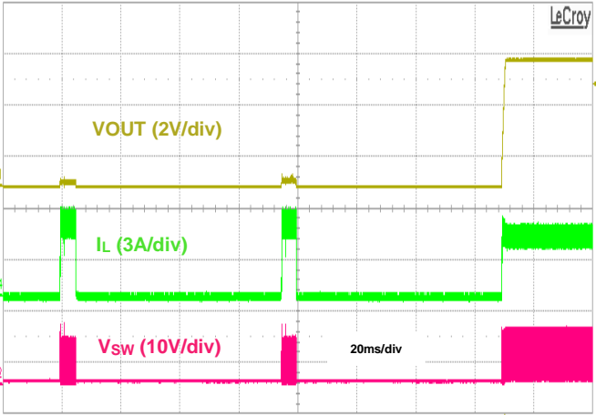
Figure 32. Output Short Recovery, IOOUT = 3.5A
