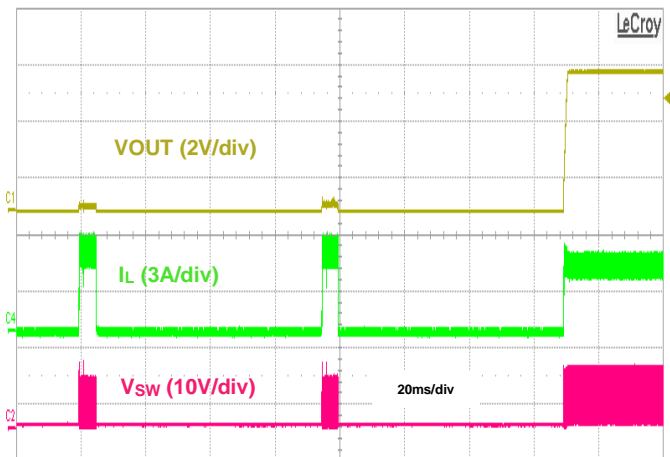
Figure 48. Output Short Recovery, I_{OUT} = 3.5\text{A}
