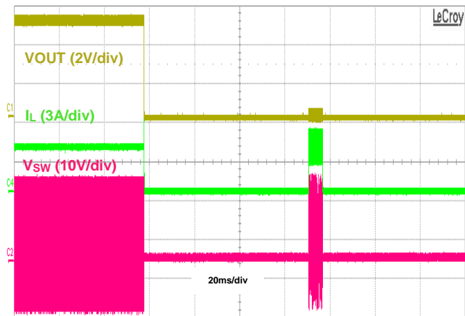
Figure 47. Output Short Protection, I_{OUT} = 3.5\text{A}
