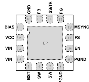
U-QFN4040-16/SWP (Type UXB)
