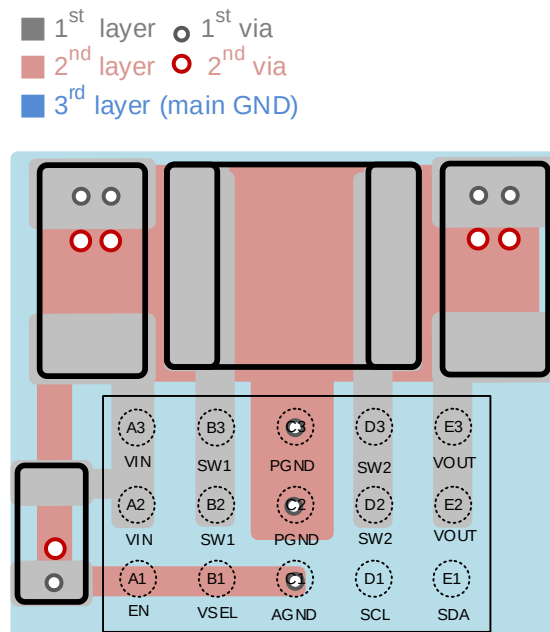
Figure 8. Layout Guide
