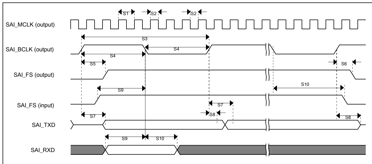
Figure 29. SAI timing—Controller modes
