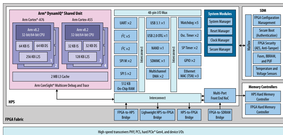
Figure 9. Agilex 5 SoCs HPS Block Diagram
