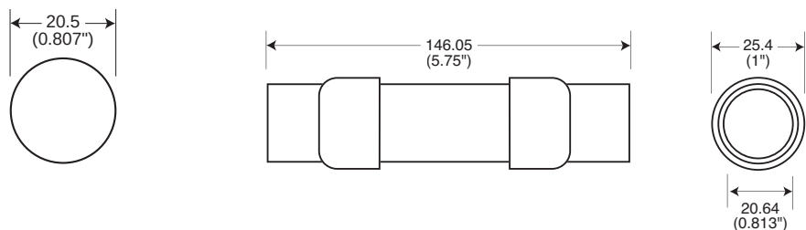
35-60A
