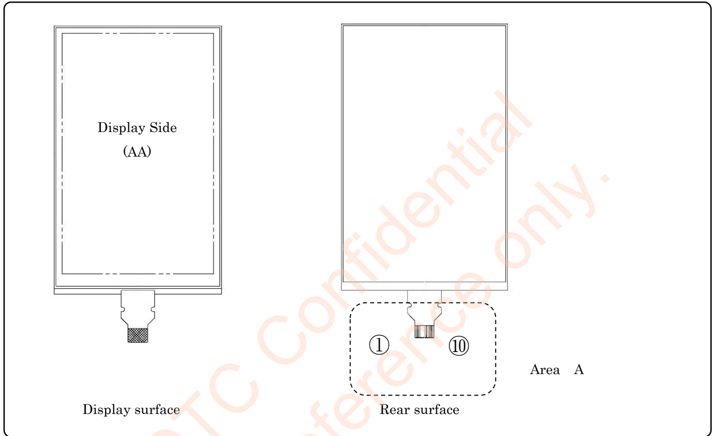
Figure 8-1-1 Pin Assignment 1
