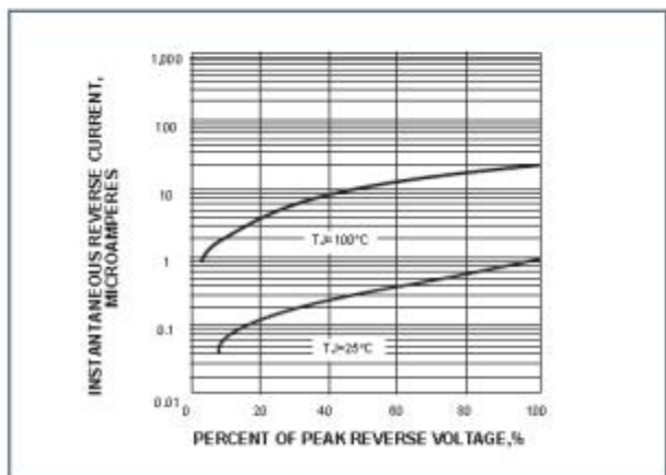
FIG. 4-TYPICAL REVERSE CHARACTERISTICS
