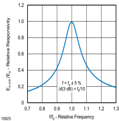
Fig. 5 - Frequency Dependence of Responsivity
