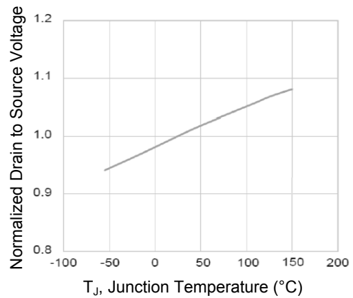
Figure 6. Normalized BV_{DSS} vs. T_J
