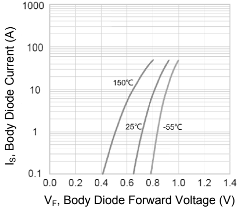
Figure 7. Body Diode Characteristics
