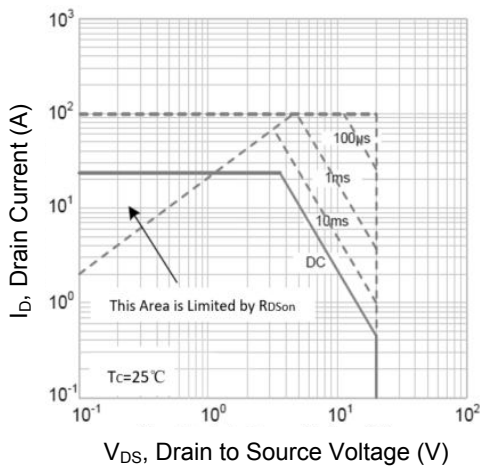
Figure 9. Safe Operation Area
