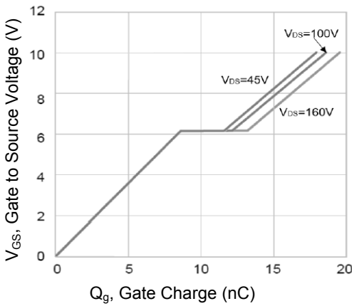
Figure 3. Gate Charge
