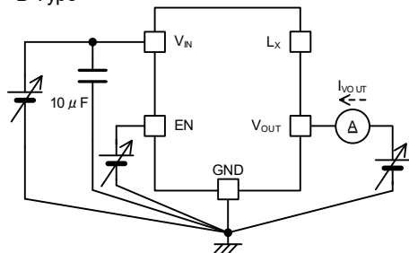
< Circuit No.7 > B Type
