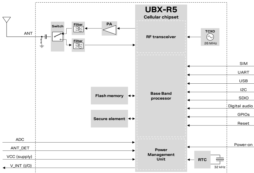
Figure 1: SARA-R510AWS block diagram
