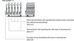
Example of a 2-pole terminal strip; with operating slot; with snap-in mounting foot Pole number = 2
