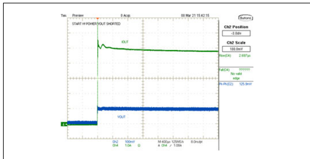
FIGURE C-17: Startup with Enable V_{OUT} = \text{Shorted to Ground} .
