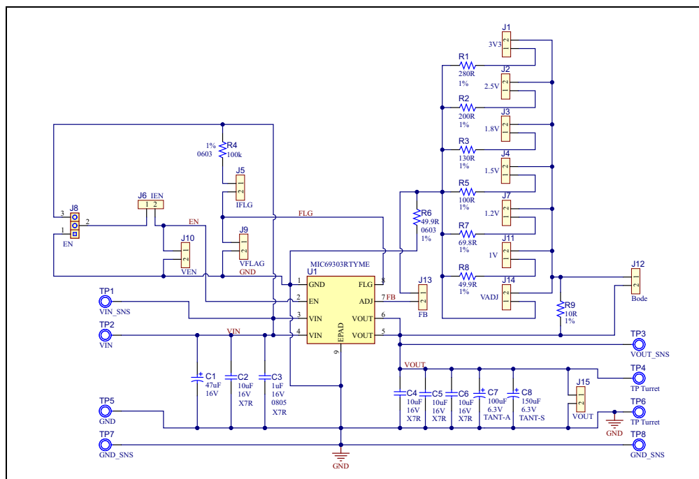
FIGURE 2-2: MIC69303RT_P-EV Evaluation Board Circuit.
