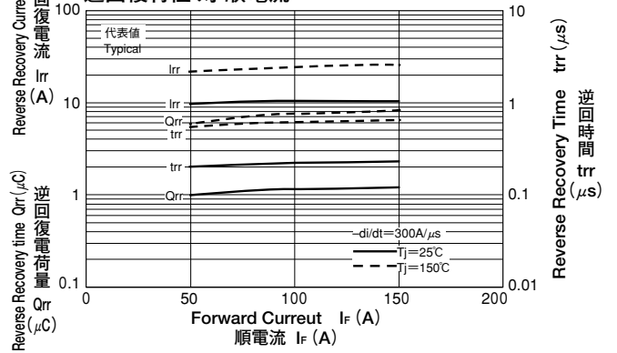
Reverse Recovery Characteristics 逆回復特性 对 順電流
