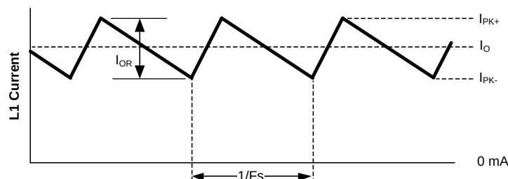
Figure 13. Inductor Current
